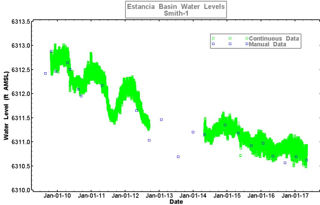
Figure 15. Water levels measured in the Smith-1 well.
