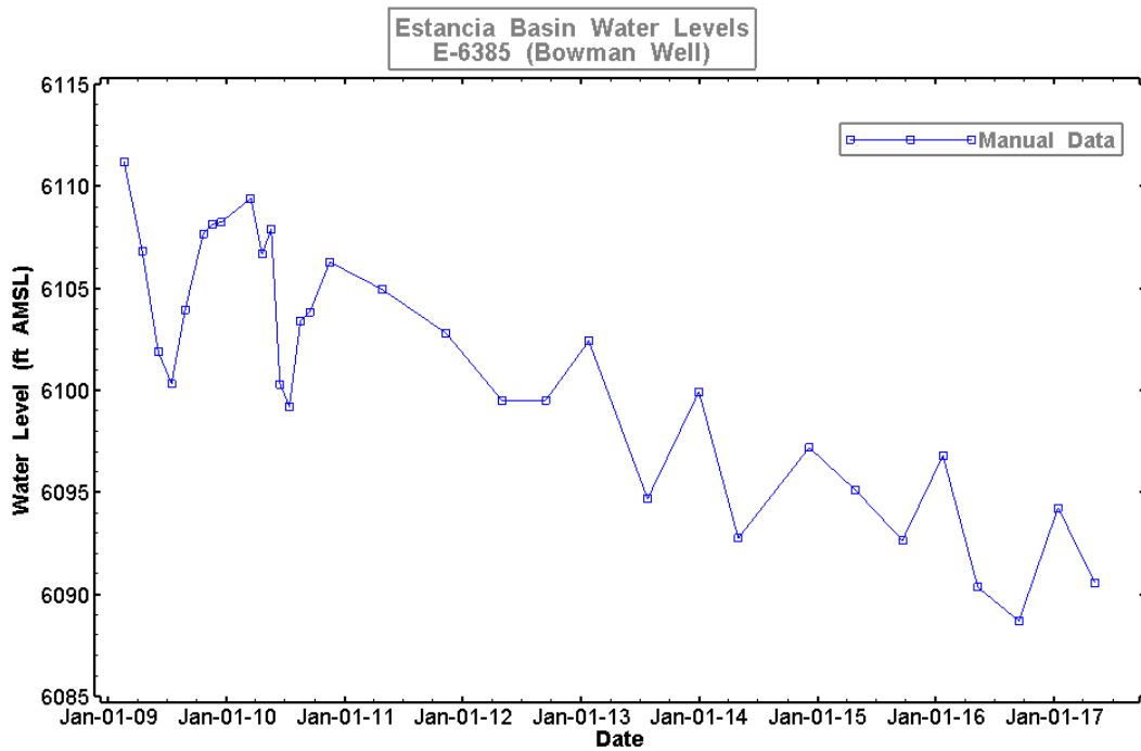
Figure 9. Water levels measured in well E-6385.
