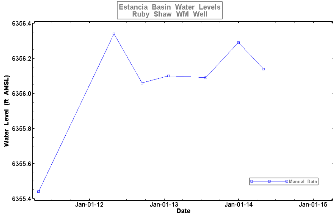
Figure 16. Water levels measured in the Ruby Shaw windmill well.
