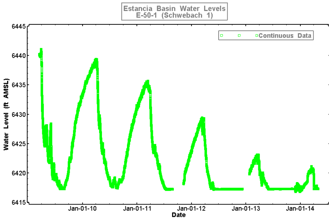
Figure 10. Water levels measured in well E-50-1.
