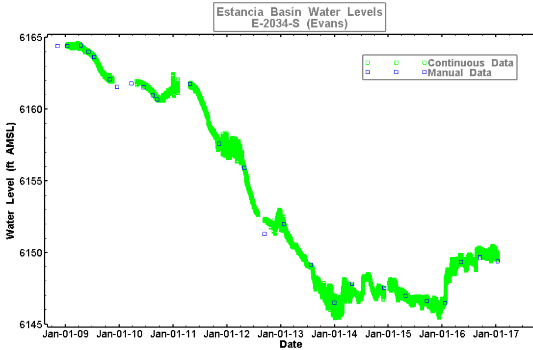
Figure 12. Water levels measured in well E-2034-S.
