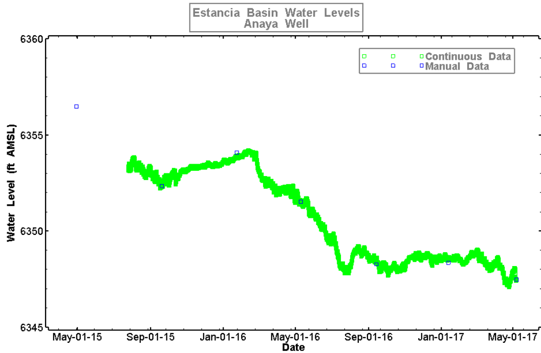
Figure 7. Water levels measured in the Anaya well.
