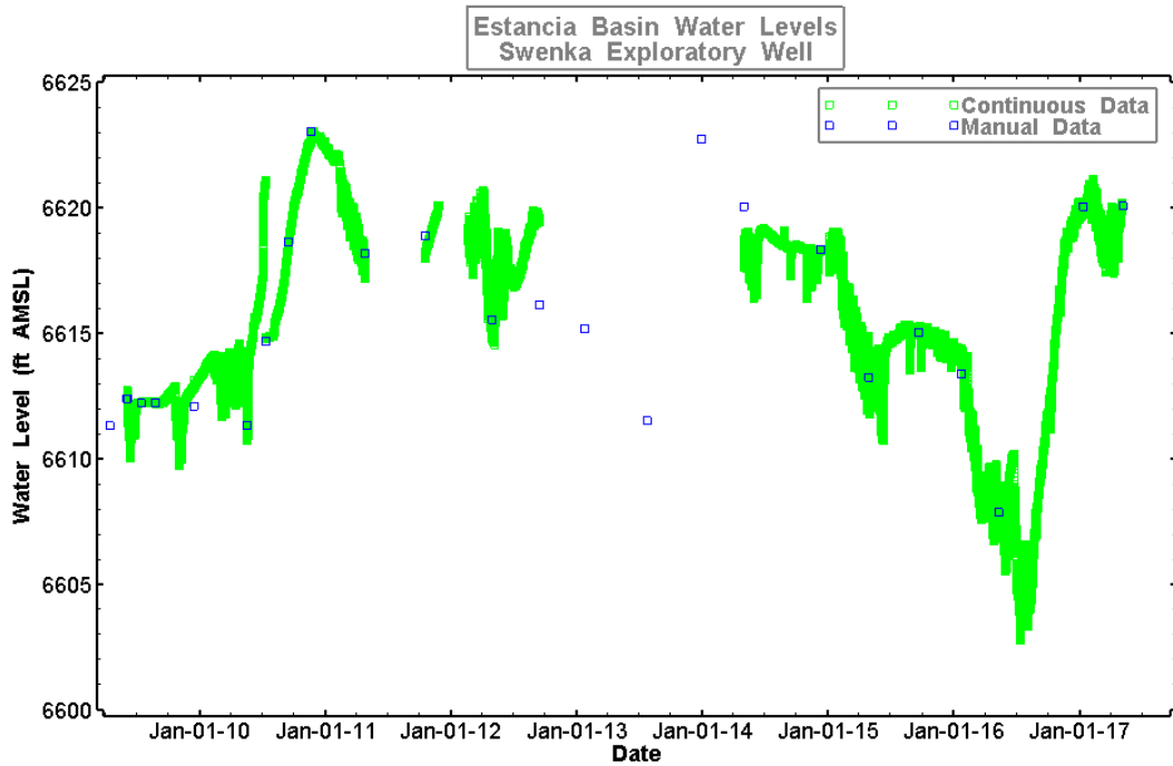
Figure 13. Water levels measured in the Swenka Exploratory well.
